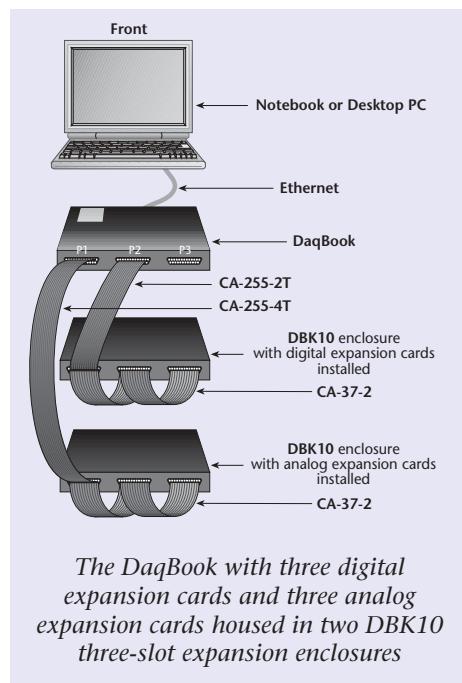
The DBK10 provides three slots for IOtech's DBK expansion cards
